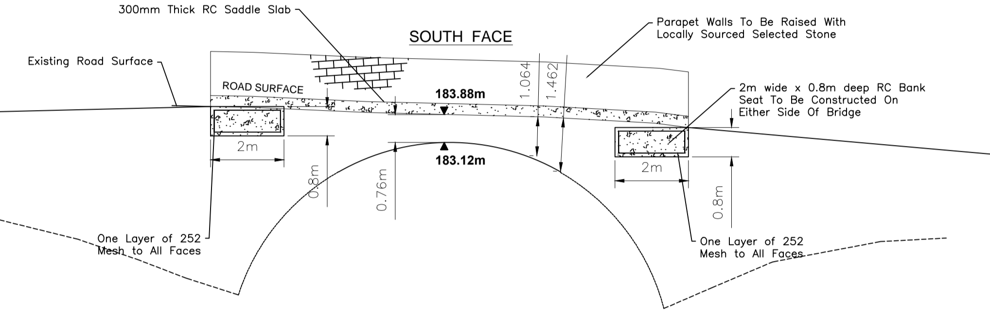
PROPOSED BRIDGE IMPROVEMENT WORKS SCALE 1:100
